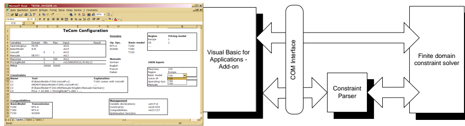
Figure 2: Architecture overview.
