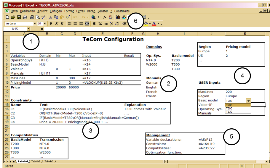
Figure 1: Application screenshot for telecommunication switch configuration
